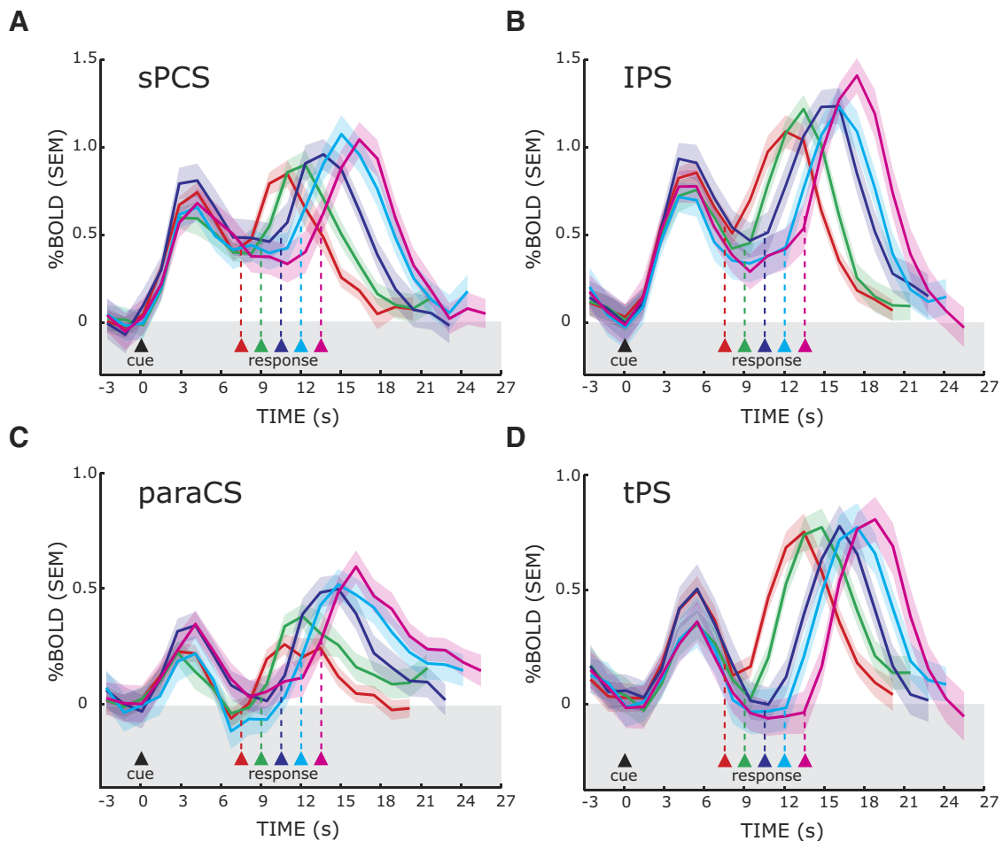
FIG. 5. Trial-averaged BOLD time courses aligned on the presentation of the instruction cue during known trials. Separate lines represent the different delay lengths, where the time of the saccade is indicated by the colored triangles and dotted lines. The data plotted are for combined contraversive pro- and antisaccades. The peaks of the responses are staggered according to the preparatory delay length. Importantly, the sPCS and IPS regions-of-interest (ROIs) showed evidence of building activity regardless of the length of the delay, even at very long delays. Each line represents the mean across subjects and the error bands are the mean of each subject's SE.
